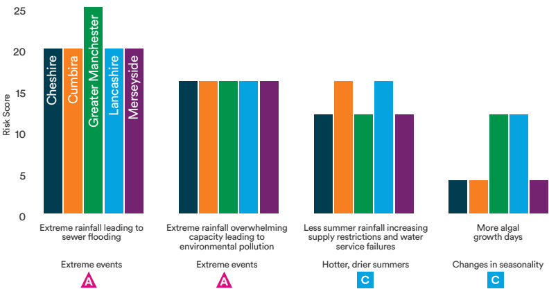
Risk scores for the top four climate risks by county
